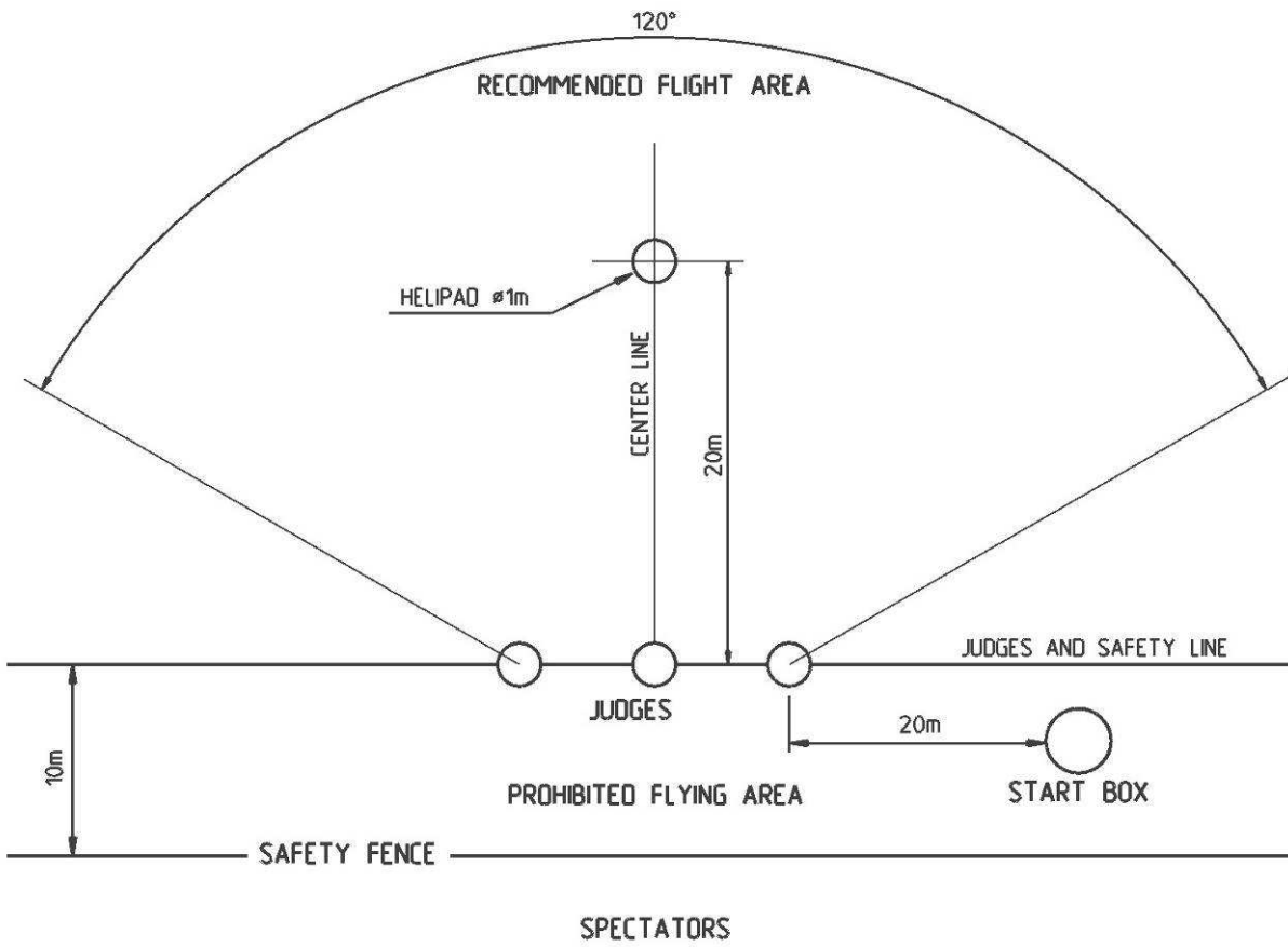
FIGURE 5.11 A – F3N CONTEST AREA LAYOUT
