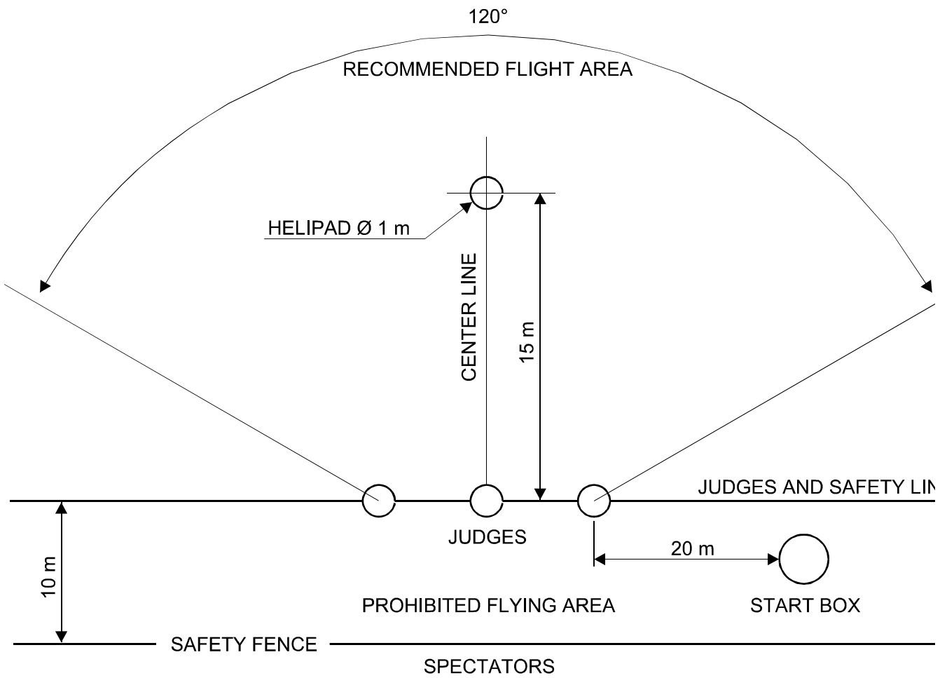
FIGURE 5F.A – F3N CONTEST AREA LAYOUT
